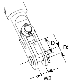
Chape standard Furlex
