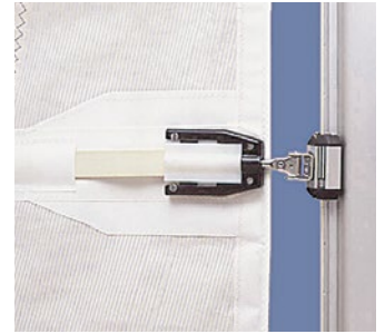
RCB batten car with M10 bolt.
