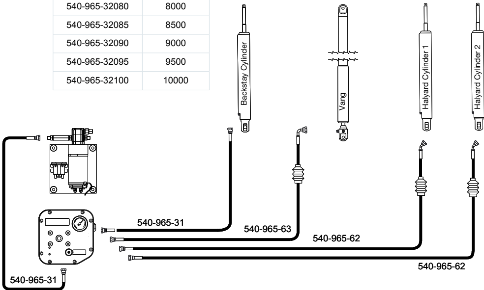
Electric pump, control panel and high-pressure hoses.
