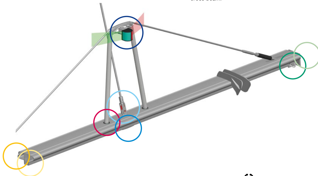
The forestay load is absorbed by a stainless support underneath the cross beam.
